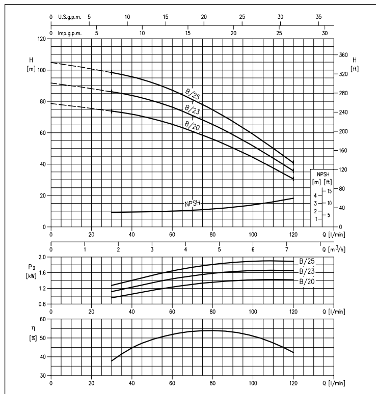
CVM B range PERFORMANCE CURVES (from 1.5 to 1.85 kW) (according to ISO 9906 Attachment A)
