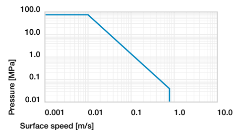
Diagram 01: Permissible pv values for iglidur® GLW plain bearings with a wall thickness of 1mm, dry operation against a steel shaft, at +20°C, mounted in a steel housing
